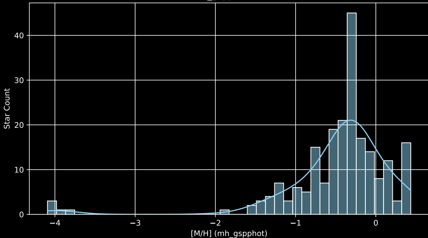
APOGEE DR17 Field: [IC348_RV [M/H] (mh_gspphot) (n= 213)
