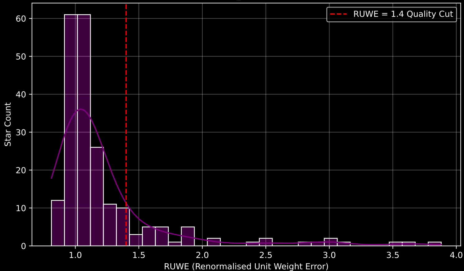
GAPOGEE DR17 Field [IC348_RV] RUWE Distribution (n= 213)
