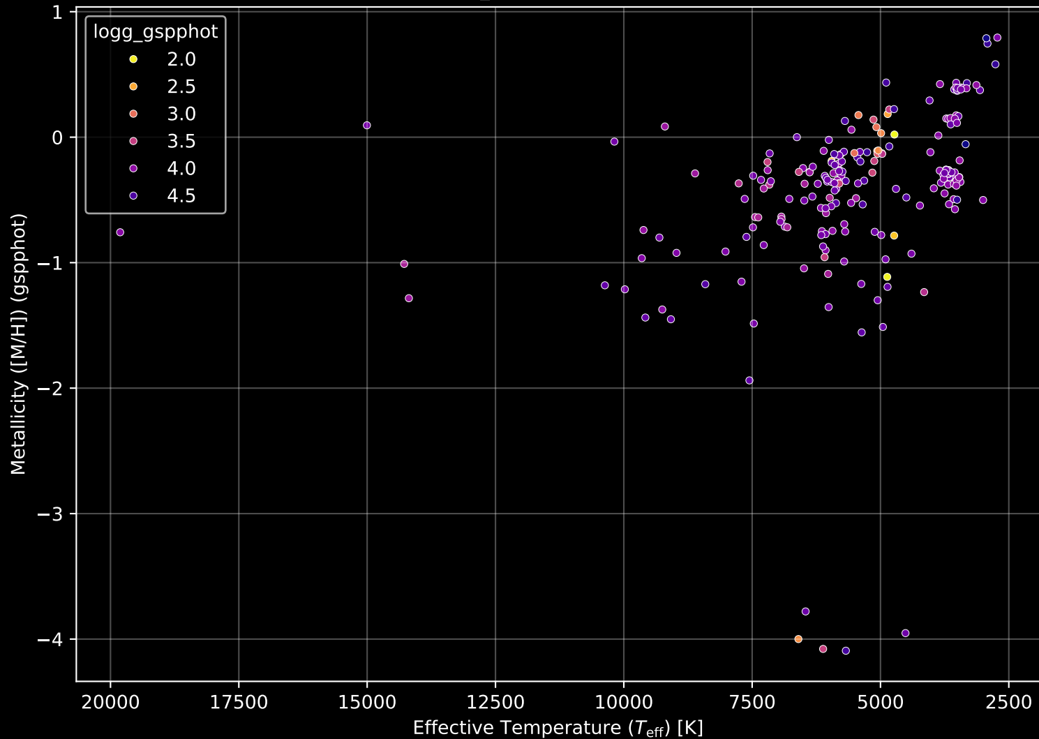
APOGEE DR17 Field: [IC348_RV] Stellar Population Parameters (n= 217)
