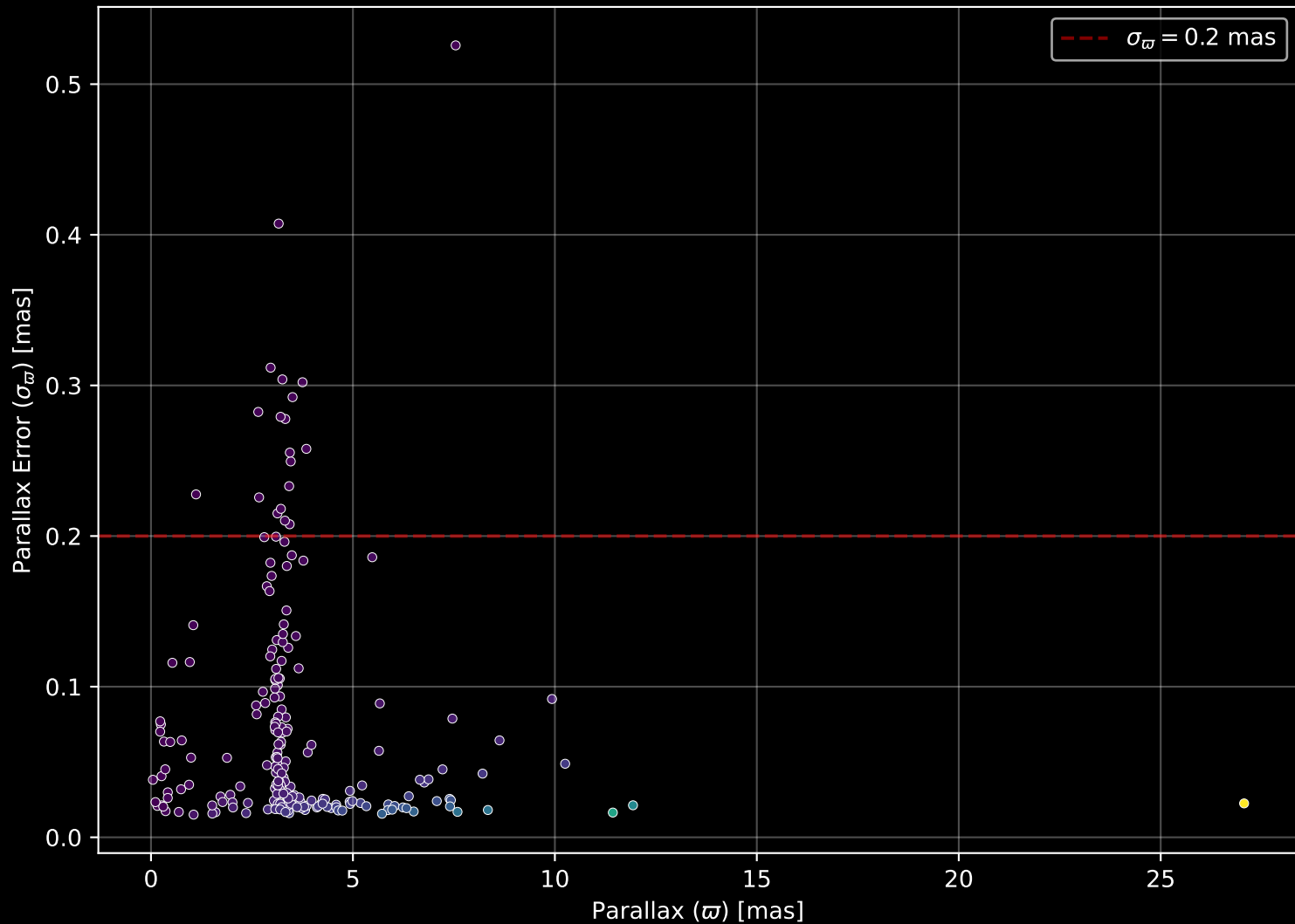
APOGEE DR17 Field: [IC348_RV] Parallax Quality (n= 217)
