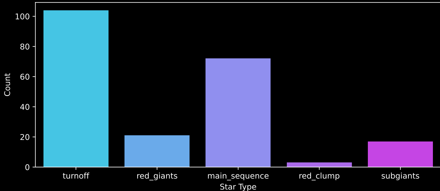
APOGEE DR17 Field: [IC348_RV] Count plot of Star Type
