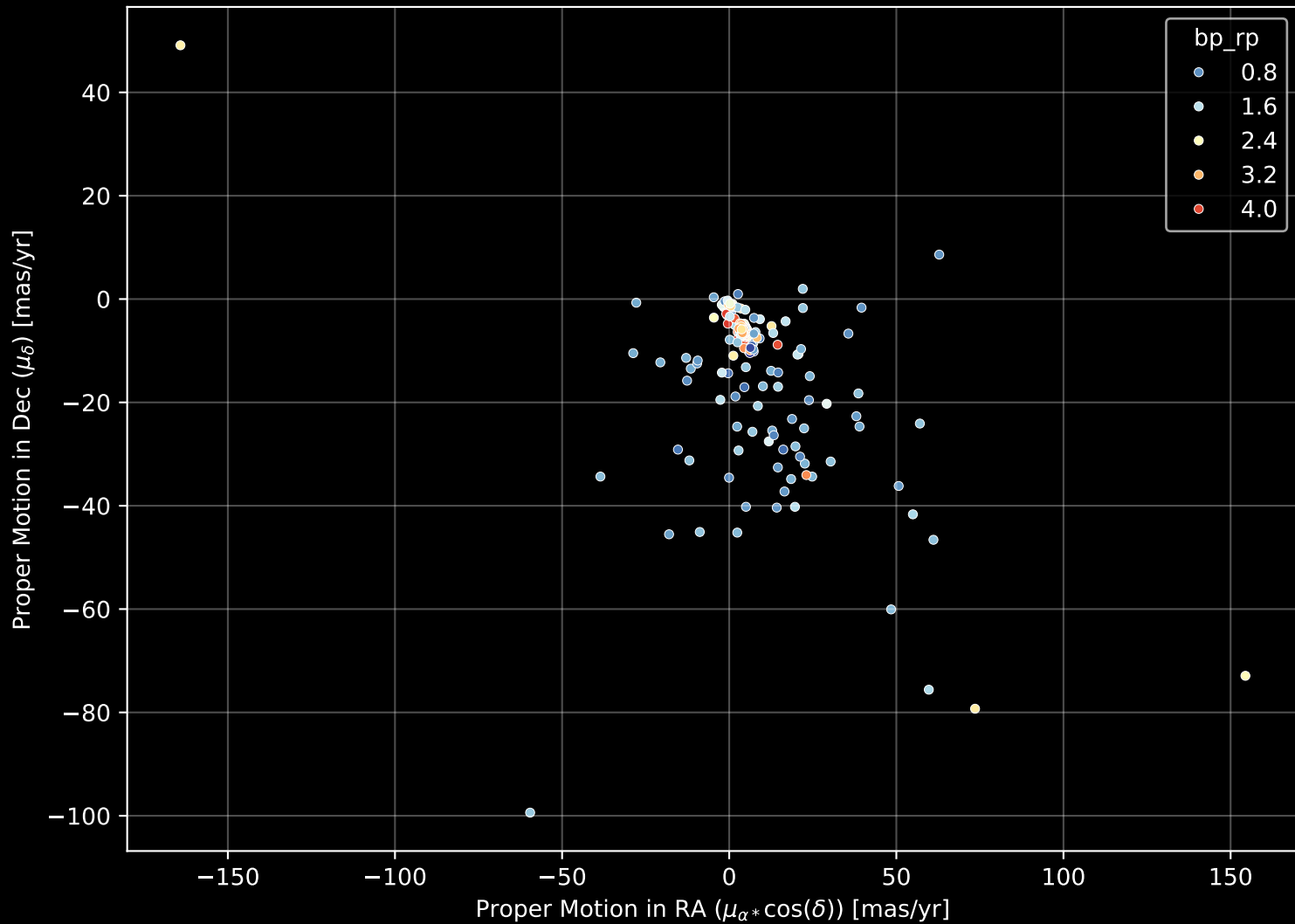
APOGEE DR17 Field: [IC348_RV] Proper Motion Diagram (n= 217)
